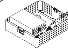
90 Amp/Hour Battery Moov-BAT-90 90 amp/hour battery, power supply, RUI and large base riser.
